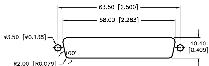
Panel Cutout
