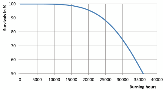
Life Expectancy Diagram - SON-T PIA PLUS 250W E E40 1SL/12
