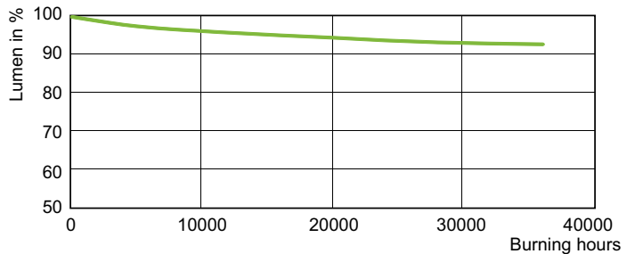
Lumen Maintenance Diagram - SON-T PIA PLUS 250W E E40 1SL/12
