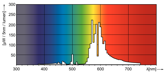
Spectral Power Distribution Colour - SON-T PIA PLUS 250W E E40 1SL/12
