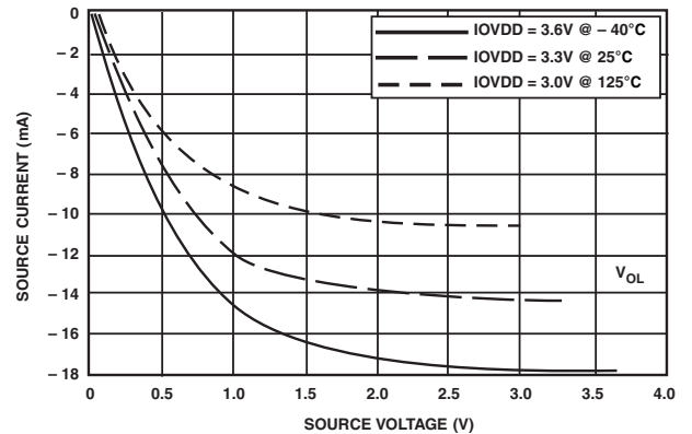
Figure 23. P_C Drivers (3.3 V IOVDD)
