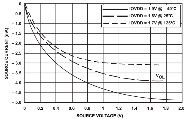
Figure 22. P_C Drivers (1.8 V IOVDD)
