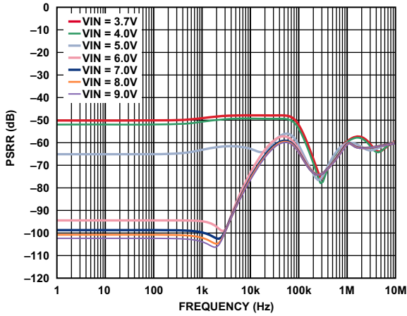
Figure 5. VOUT1 PSRR, I_{\text{OUT1}} = 10\ \text{mA}
