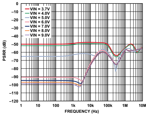
Figure 6. VOUT1 PSRR, I_{\text{OUT1}} = 40\ \text{mA}
