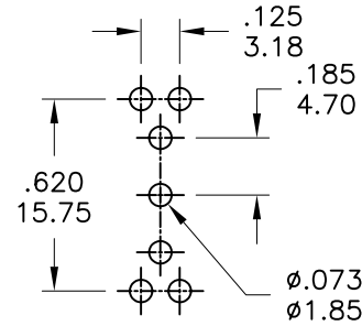
P.C. MOUNTING
