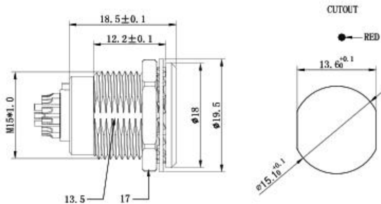
CONNECTOR SIDE VIEW
