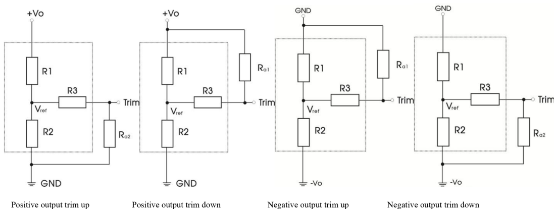
Fig.4 Circuit diagram of Vtrim up and down (dashed line shows internal part of module)
