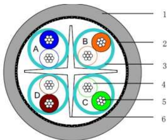
Cross Section
