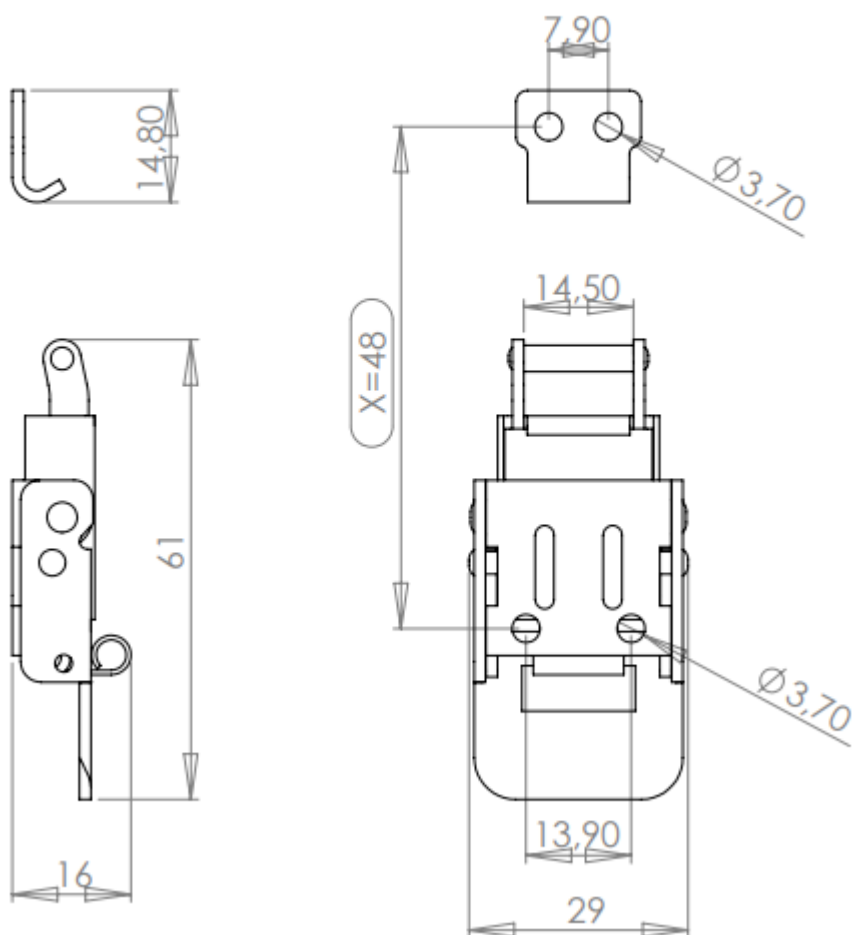
7264169 S Steel Catch Plate
