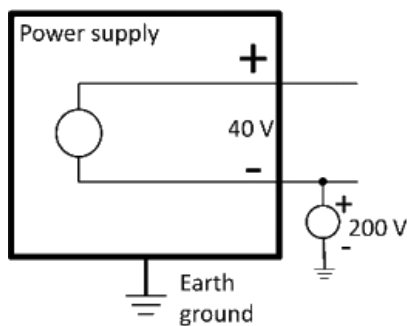
Example of negative terminal floating +200 V above ground (positive terminal is +240 V above ground)
