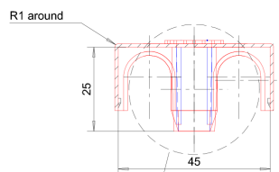
Section B - B M 3:1
