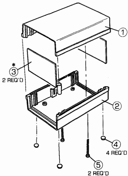
MODEL CM3-150 STANDARD
