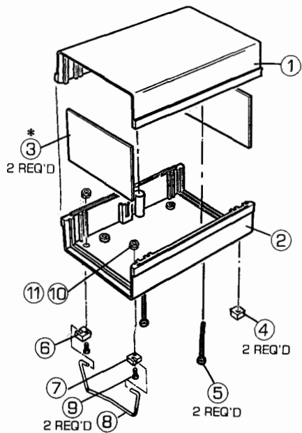
MODEL CMB3-150 BAILED
