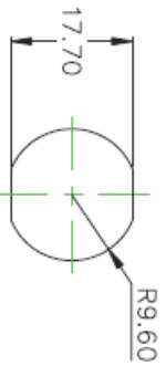
PANEL CUTOUT MAX. PANEL THICKNESS: 10.0mm
