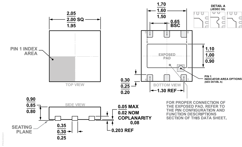
Figure 83. 6-Lead Lead Frame Chip Scale Package [LFCSP] 2 mm x 2 mm Body and 0.85 mm Package Height (CP-6-12) Dimensions shown in millimeters
