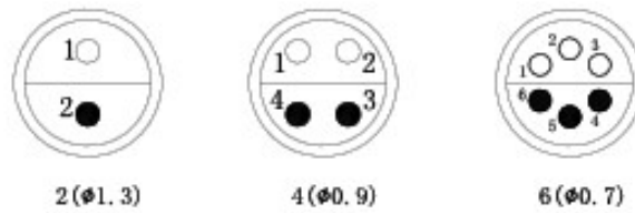
CONNECTOR SOLDER CUP VIEW
