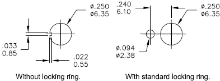
PANEL MOUNTING
