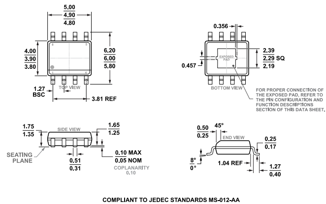
Figure 68. 8-Lead Standard Small Outline Package, with Exposed Pad [SOIC_N_EP] Narrow Body (RD-8-1) Dimensions shown in millimeters
