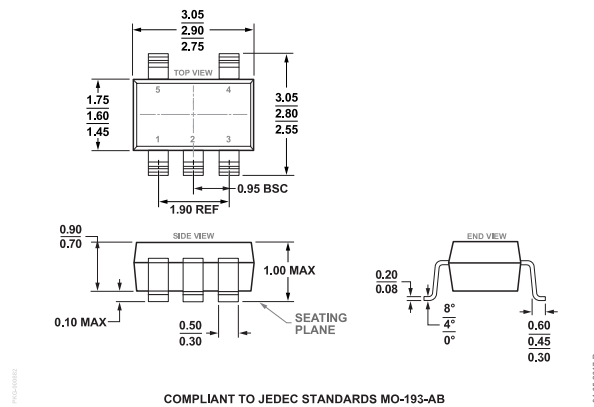
Figure 69. 5-Lead Thin Small Outline Transistor Package [TSOT] (UJ-5) Dimensions shown in millimeters
