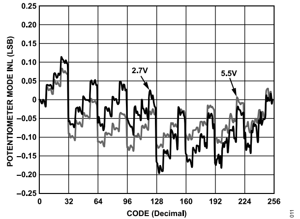
Figure 10. INL vs. Supply Voltages
