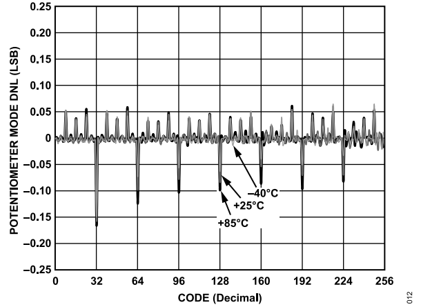
Figure 9. DNL vs. Code vs. Temperature
