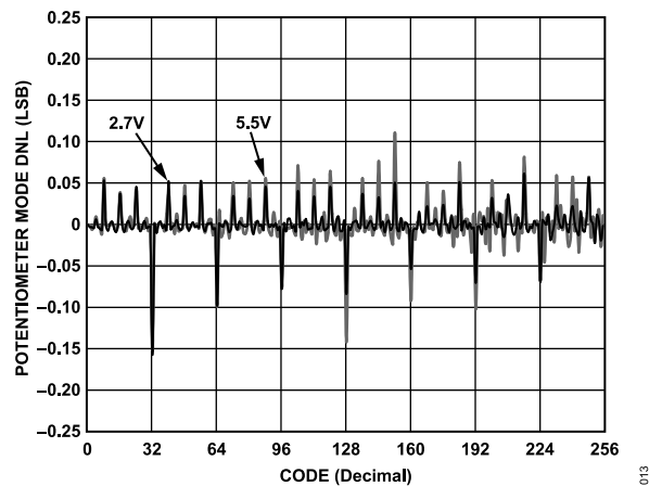
Figure 11. DNL vs. Code vs. Supply Voltage
