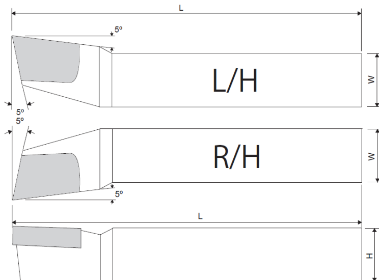
Carbide Tipped Lathe Tools Cranked Knife/Turning Tools ISO-3
