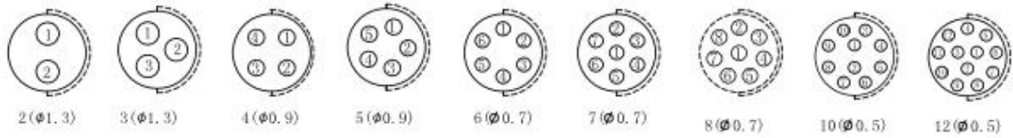
CONNECTOR SOLDER CUP VIEW
