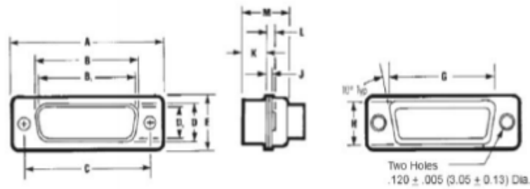
Mating Side
