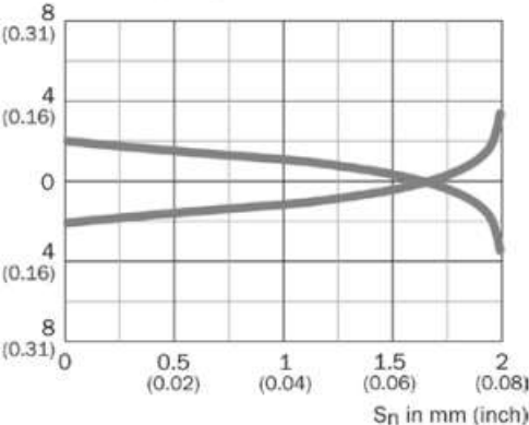
Response diagram
