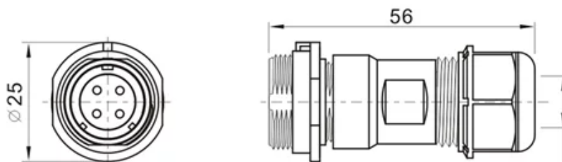
Cable outer diameter range: 6-10mm
