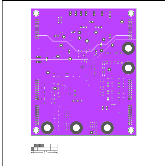
MAX15157D EV Kit PCB Layout—Layer 5
