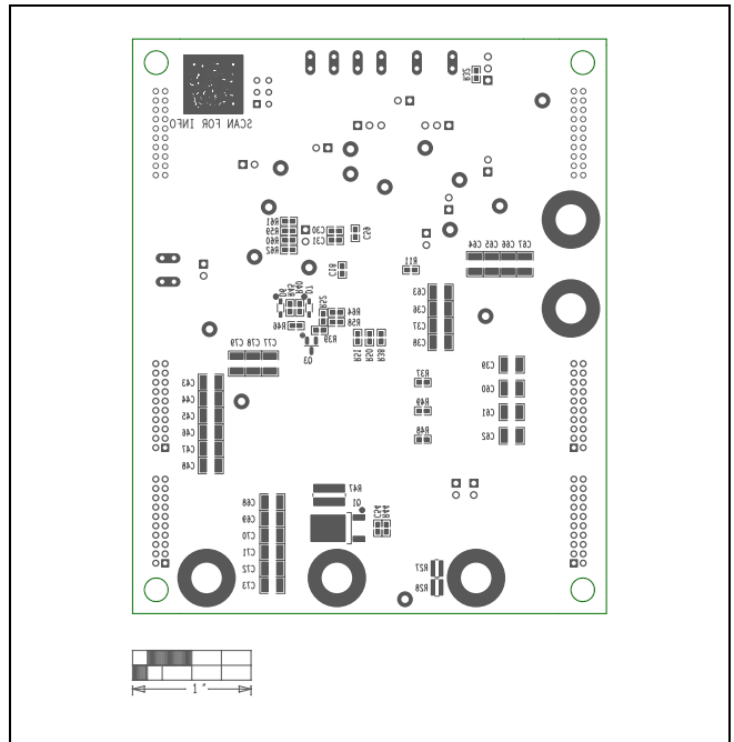
MAX15157D EV Kit Component Placement Guide—Bottom Silkscreen
