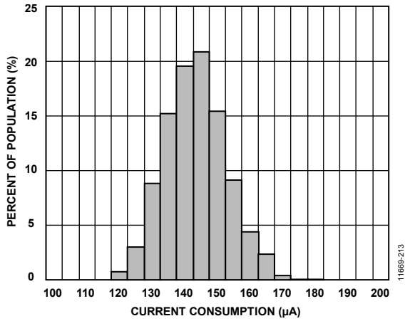
Figure 17. Current Consumption at 25°C, 100 Hz Output Data Rate, V_s = 2.5\text{ V}
