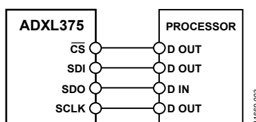
Figure 23. 4-Wire SPI Connection Diagram
