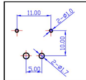
Installation hole diagram
