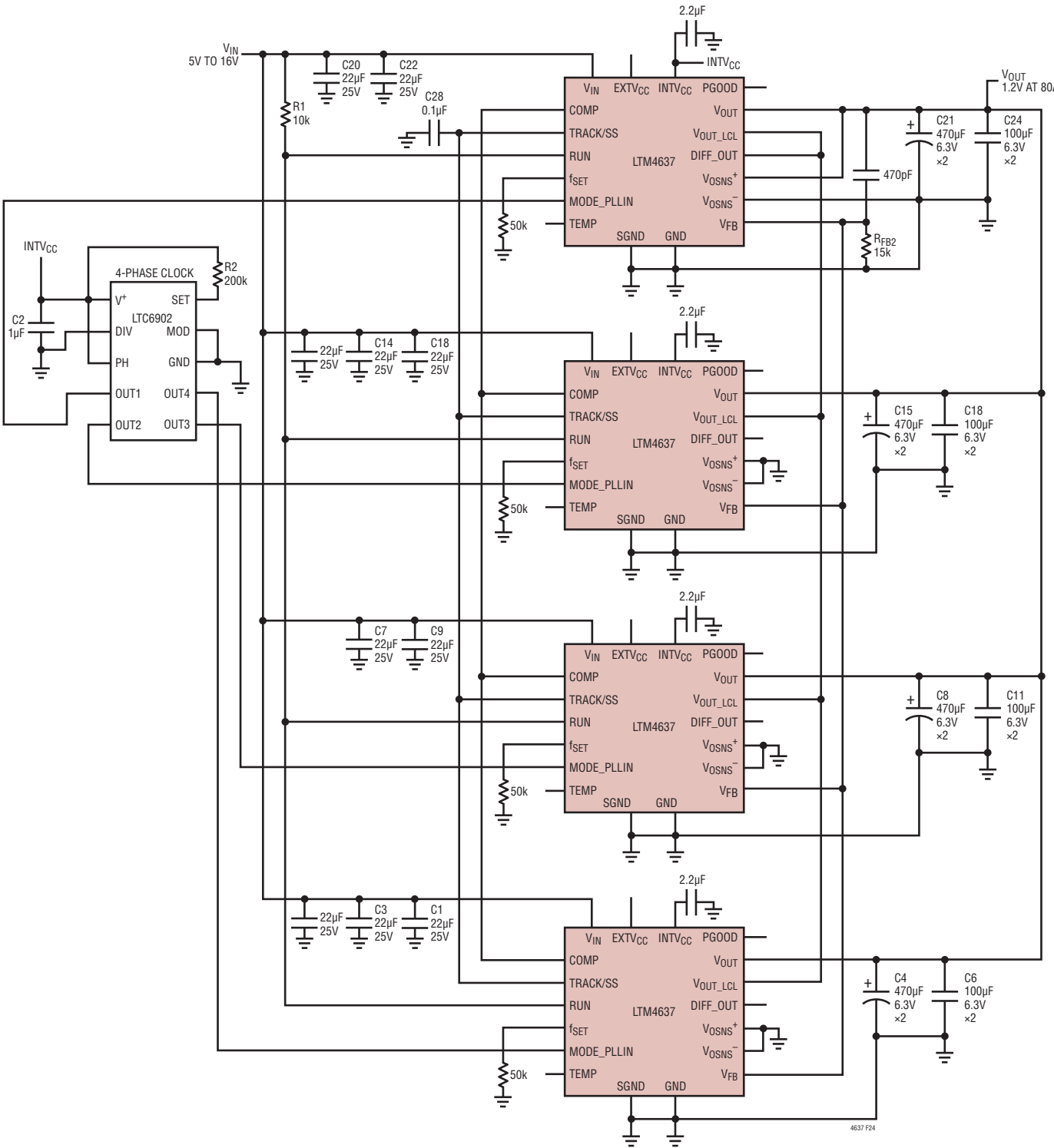
Figure 24. 1.2V, 80A, Current Sharing with 4-Phase Operation
