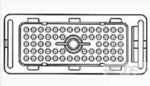
TE Part #211580-5 MMATE,RCPT,62P,PSTD LF
