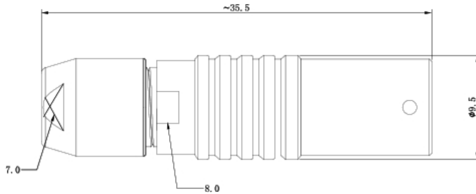
CONNECTOR SOLDER CUP VIEW
