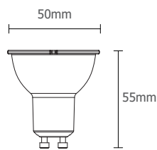
PAR16S1-7.2W-F-GU10
