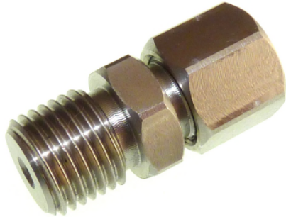
(BSP parallel example - 381-7362, see below for other sizes)
