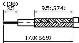
STRIPPING DIMENSION SCALE 3:1
