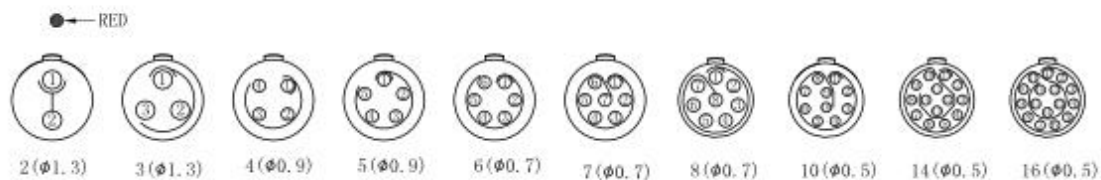
CONNECTOR SOLDER CUP VIEW
