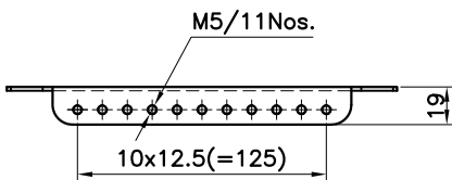
DETAIL OF MOUNTING RAIL
