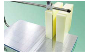
Straight line cutting of a thick material using a angle square
