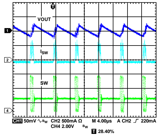
Figure 20. Typical Waveforms, V_{OUT2}=1.8\text{ V} , I_{OUT2}=30\text{ mA} , Automatic Mode
