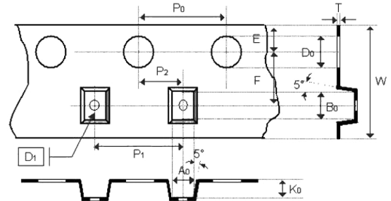
The dimension of plastic tape
