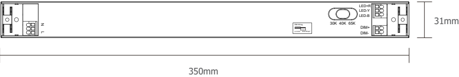
LED Driver
