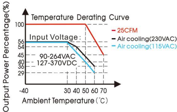
2367920, 2367924 Input Voltage Derating Curve
