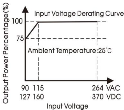
2367920, 2367924 Input Voltage Derating Curve
