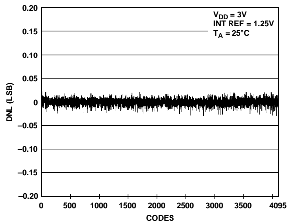
Figure 17. DNL AD5629R-1—Internal Reference
