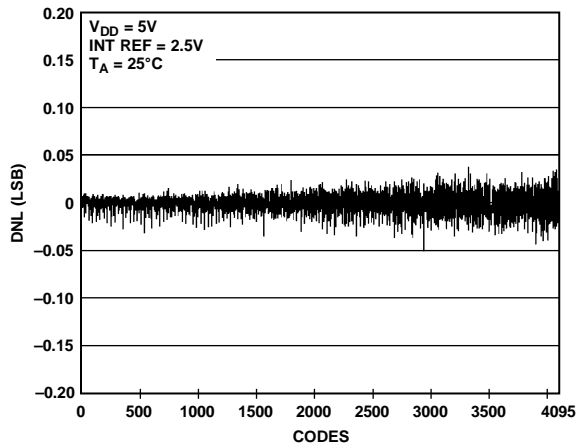
Figure 13. DNL AD5629R-2—Internal Reference
