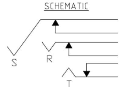
STEREO (BBB) JACK SWITCH CONTACTS OPEN WHEN PLUG IS INSERTED + CLOSE WHEN PLUG IS WITHDRAWN.
