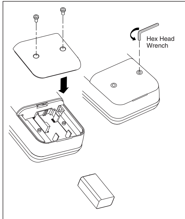
Figure 7. Battery Replacement
