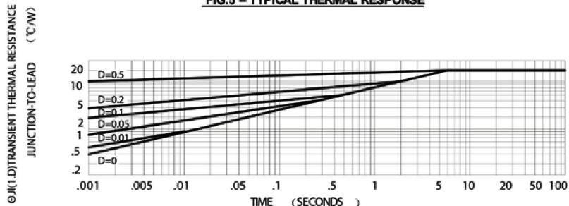
FIG.5 – TYPICAL THERMAL RESPONSE
