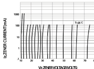
FIG.8 – ZENER VOLTAGE VERSUS ZENER CURRENT Vz=11 THRU 75 VOLTS
