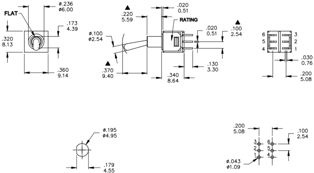
P.C. MOUNTING
