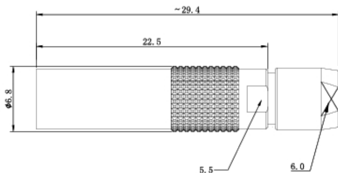
CONNECTOR SOLDER CUP VIEW
