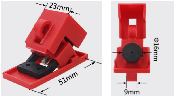
CB011(X) 959431(X) Clamp-on Circuit Breaker Lockout Small Toggle Up to 18mm
