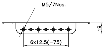
DETAIL OF MOUNTING RAIL
