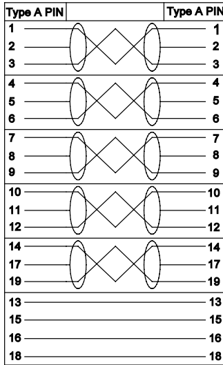
Wire method
