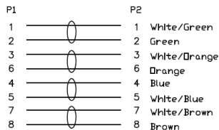
PIN ASSIGNMENT (TIA 568A)
