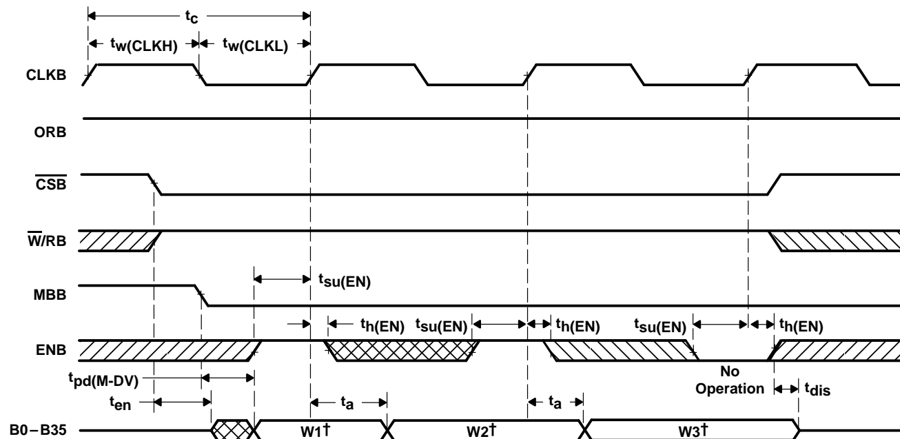
Figure 6. Port-B Read-Cycle Timing for FIFO1
