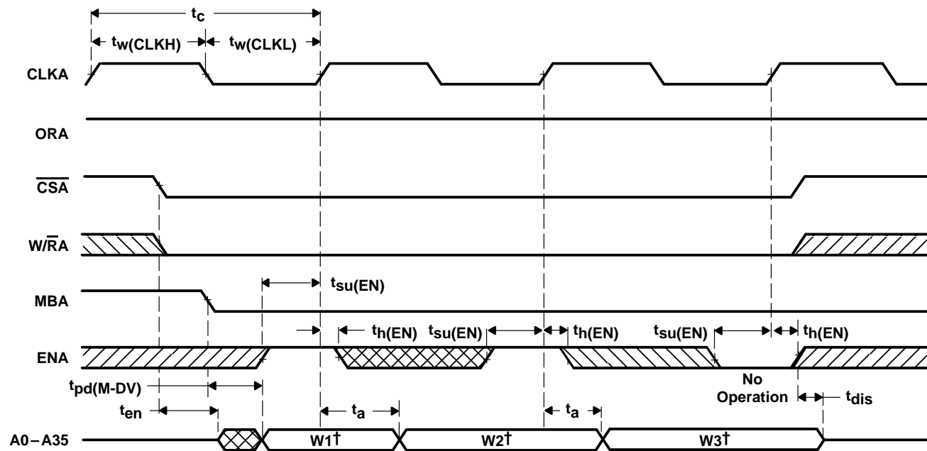
Figure 5. Port-A Read-Cycle Timing for FIFO2
