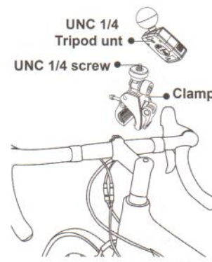
Fig. 8 Bike application
