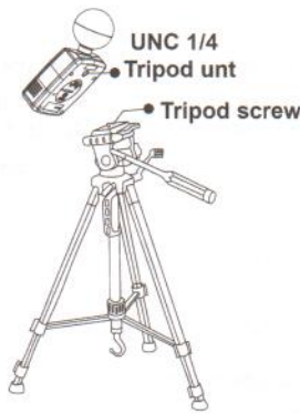
Fig. 7 Tripod application
